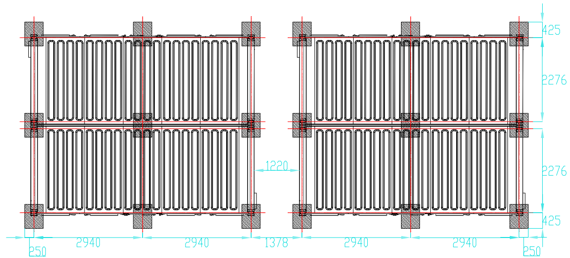
PLAN - FOUNDATIONS
